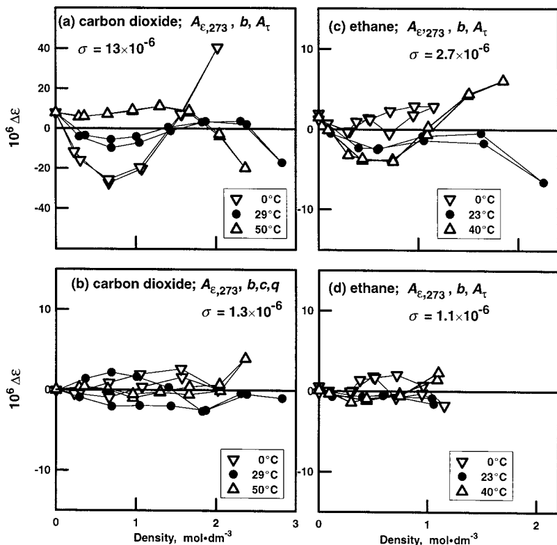
Fig. 7. Deviations of \epsilon(p, T) data from Eq. (7). (a) Three-parameter fit for carbon dioxide. (b) Five-parameter fit for carbon dioxide. (c) Three-parameter fit for ethane. (d) Three-parameter fit for the lowest-density data for ethane.
