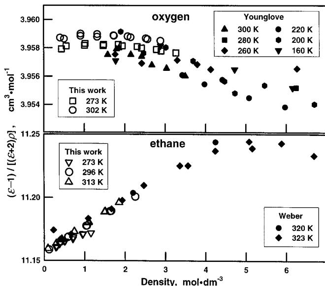
Fig. 9. Comparison of oxygen and ethane results with data from the literature. Oxygen: The open symbols represent the present data; the filled symbols represent the data of Younglove [18]. The values of (\epsilon-1)/[(\epsilon+2)\rho] were calculated using the equation of state from Ref. 15. Ethane: The open symbols represent the present data; the filled symbols represent the data of Weber [31]. The values of (\epsilon-1)/[(\epsilon+2)\rho] were calculated using the equation of state from Ref. 24.
